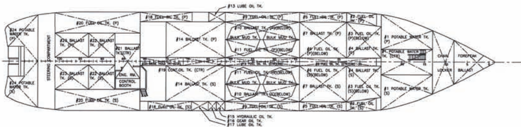
HOLD PLAN
