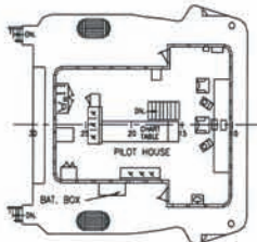
PILOT HOUSE
