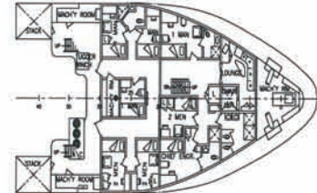
CABIN DECK
